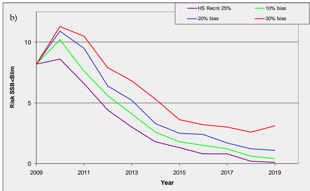
Figure 5.8.2.2. Herring in VIa (N). Risk of SSB < B_{lim} under different model conditions. Results of medium term simulations of EC harvest rule (see Section 5.1.3.), for model parameters given in section 5.8. a) Sensitivity to 20/25% year-on-year constraint on TAC change (dotted / solid lines). Sensitivity to choice of S/R model; Hockey-Stick (runs 9, 10, 11, 12) Beverton-Holt (runs 5, 6, 7, 8). Sensitivity to choice of measurement error (CV of 25% runs 9, 10, 5, 6 or 30% runs 11, 12, 7, 8) b) Sensitivity to over catch 0, 10, 20, 30% bias for the case of the HS model runs 6, 13, 14, 15. In all cases risks fall below 5% but at 30% bias (overcatch) risks are no longer negligible.
