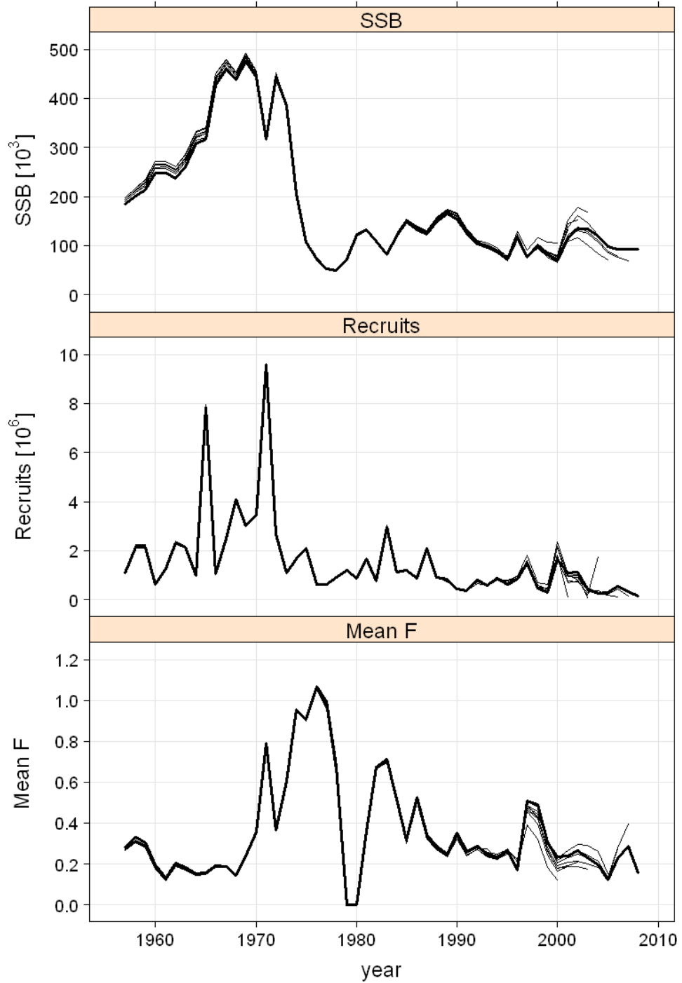
Figure 5.6.2.13. Herring in VIa (N). Analytical retrospective patterns (2008 to 2001) of SSB, mean F_{3-6} and recruitment from the final assessment.
