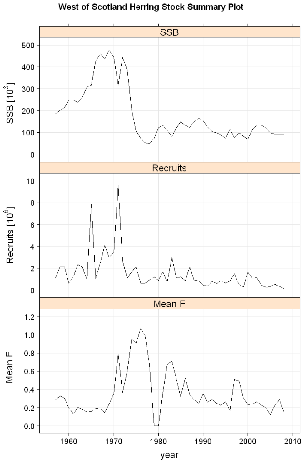
Figure 5.6.2.1. Herring in VIa (N). Illustration of stock trends from the assessment (8 year separable period) 1957-2008. Summary of estimates of landings, spawning stock biomass at spawning time, fishing mortality at F_{3-6} , recruitment at 1-ring, in the final assessment run.
