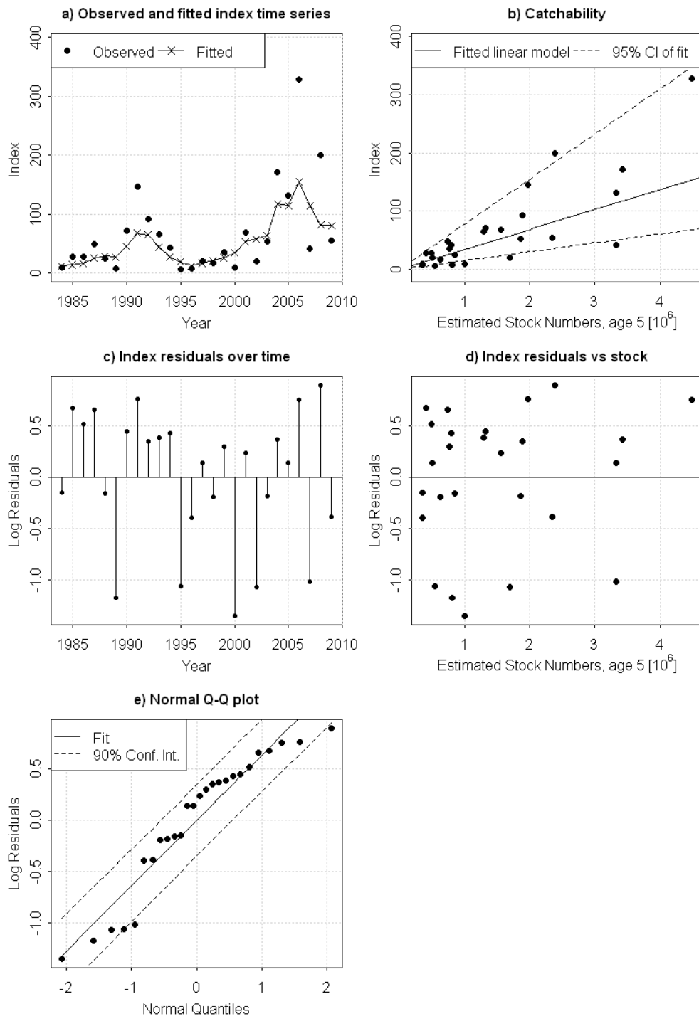
Figure 2.6.1.14. North Sea herring. Diagnostics of IBTS survey catchability at 5+ wr from the final ICA assessment. Top left: VPA estimates of numbers at 5+ wr (line) and numbers predicted from index abundance at 5+ wr. Top right: scatterplot of index observations versus VPA estimates of numbers at 5+ wr with the best-fit catchability model (linear function). Middle right: log residuals of catchability model by VPA estimate of numbers at 5+ wr. Middle left: log residuals of catchability model by year. Bottom left: normal Q-Q plot of log residuals.
