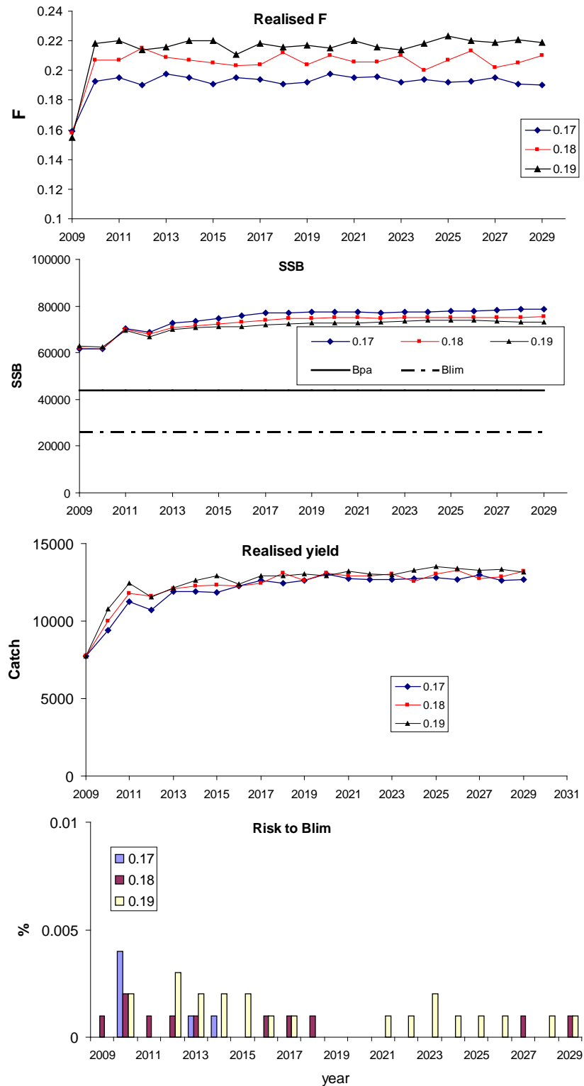
Figure 7.1. Trajectory plots for simulations of proposed rebuilding plan (Run 3). Simulated trajectories for F, SSB, catch and risk to B_{lim} . Risk to B_{lim} presented as a histogram because of very low levels.
