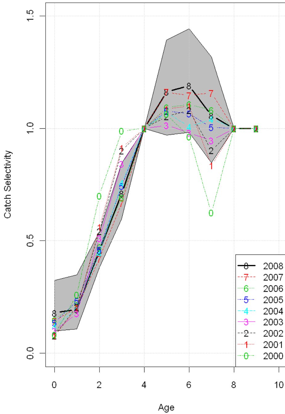
Figure 2.6.1.19. North Sea herring. Retrospective selectivity pattern for the year 2000 till 2008.
