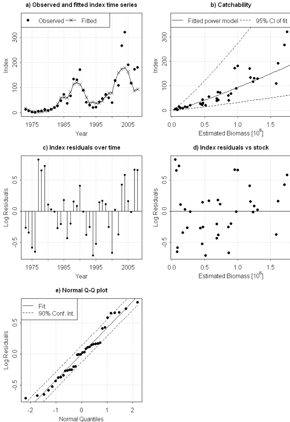
Figure 2.6.1.16. North Sea herring. Diagnostics of MLAI survey catchability at all ages from the final ICA assessment. Top left: VPA estimates of biomass of all ages and biomass predicted from index abundance for all ages. Top right: scatterplot of index observations versus VPA estimates of all ages with the best-fit catchability model (power function). Middle left: log residuals of catchability model by VPA estimate of numbers at 0 yr. Middle right: log residuals of catchability model by year. Bottom left: normal Q-Q plot of log residuals.
