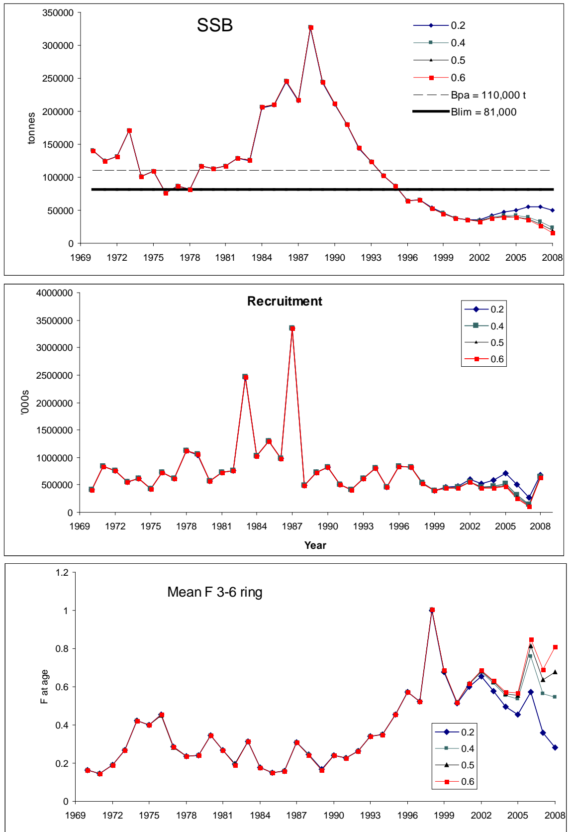
Figure 6.6.2.1. VIa(S) and VIb,c four separable VPA runs using values of 0.2, 0.4, 0.5 and 0.6 for terminal F.
