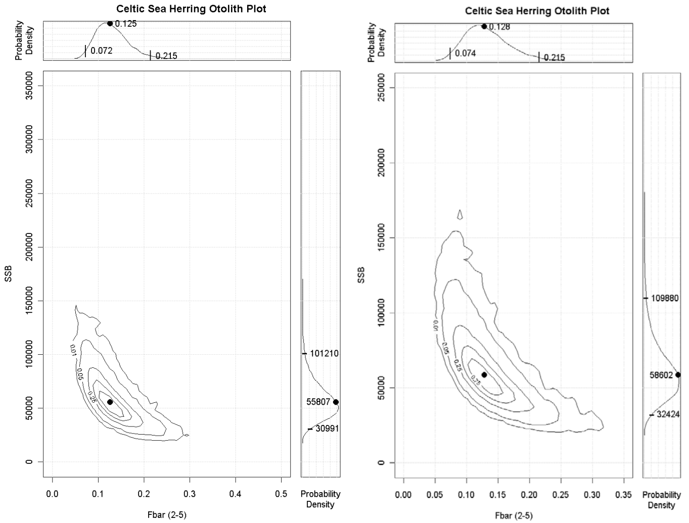
Figure 4.6.1.5. Celtic Sea and VIIj herring. Results of parametric bootstrapping from FLICA for the 6+ assessment (left) and 7+ (right).
