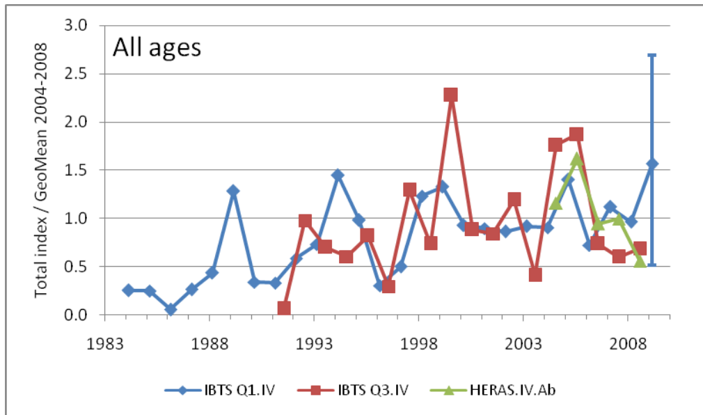
Figure 8.3.3 North Sea sprat. Normalized IBTS Q1, Quarter 3 and HERAS acoustic survey indices for the abundance of North Sea sprat. All indices are normalized by their geometric mean over the common period from 2004-2008. For the IBTS survey in Q1-2009 the standard deviation is presented with error bars.
