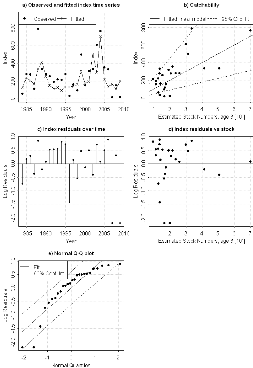
Figure 2.6.1.12. North Sea herring. Diagnostics of IBTS survey catchability at 3 wr from the final ICA assessment. Top left: VPA estimates of numbers at 3 wr (line) and numbers predicted from index abundance at 3 wr. Top right: scatterplot of index observations versus VPA estimates of numbers at 3 wr with the best-fit catchability model (linear function). Middle right: log residuals of catchability model by VPA estimate of numbers at 3 wr. Middle left: log residuals of catchability model by year. Bottom left: normal Q-Q plot of log residuals.
