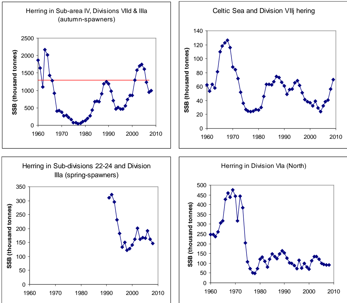
Figure 1.11.2 Spawning stock biomass estimates of the 4 herring stocks for which analytical assessments were presented in HAWG 2009. The B_{pa} level (if defined) is indicated in the graphs.
