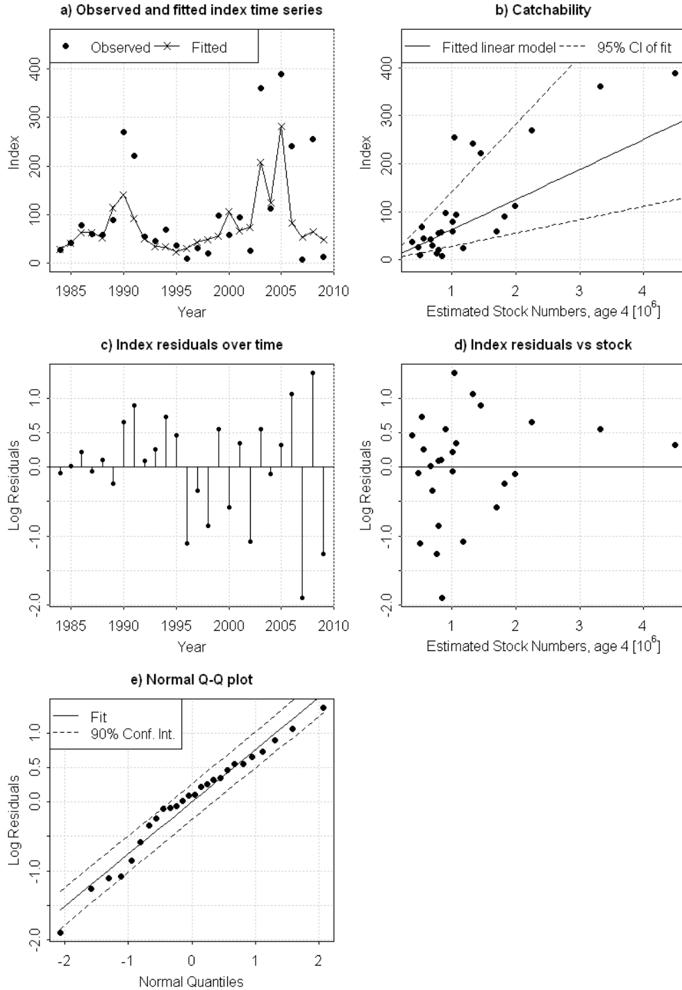
Figure 2.6.1.13. North Sea herring. Diagnostics of IBTS survey catchability at 4 wr from the final ICA assessment. Top left: VPA estimates of numbers at 4 wr (line) and numbers predicted from index abundance at 4 wr. Top right: scatterplot of index observations versus VPA estimates of numbers at 4 wr with the best-fit catchability model (linear function). Middle right: log residuals of catchability model by VPA estimate of numbers at 4 wr. Middle left: log residuals of catchability model by year. Bottom left: normal Q-Q plot of log residuals.
