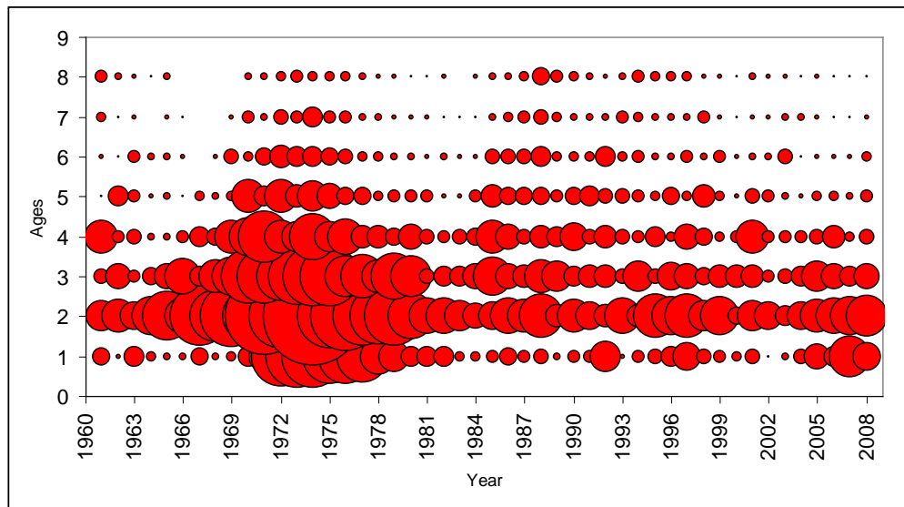
Figure 7.2.1 Irish Sea herring VIIa(N). Landings (catch-at-age) of herring from VIIa(N) from 1961 to 2008.
