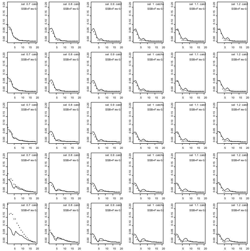
Figure 5.6.1.1. Herring in VIa (N). Mean squared deviance (y axis) between previous and current assessments for the 8 assessment years in the retrospective and years (x axis) previous to the terminal year in the assessment. 2008 WG data with flat weighting at age. SSB (dots) and F_{3-6} (solid line). Across rows selection at oldest age ranging from 0.7 to 1.2, down columns weighting on catch from 2.0 to 0.5. Minimum is candidate for best settings (see text table section 5.6.1)
