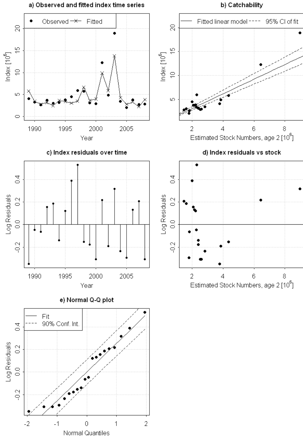
Figure 2.6.1.2. North Sea herring. Diagnostics of Acoustic survey catchability at 2 wr from the final ICA assessment. Top left: VPA estimates of numbers at 2 wr (line) and numbers predicted from index abundance at 2 wr. Top right: scatterplot of index observations versus VPA estimates of numbers at 2 wr with the best-fit catchability model (linear function). Middle right: log residuals of catchability model by VPA estimate of numbers at 2 wr. Middle left: log residuals of catchability model by year. Bottom left: normal Q-Q plot of log residuals.
