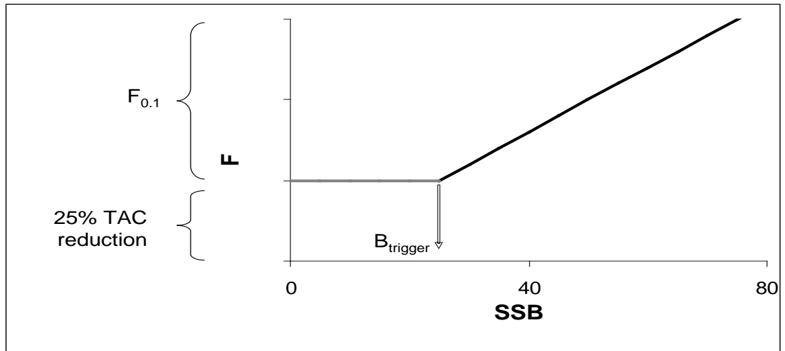
Figure 1. Schematic representation of the decision rule in the proposed rebuilding plan. B_{trigger} = B_{lim} = 26,000 t.
