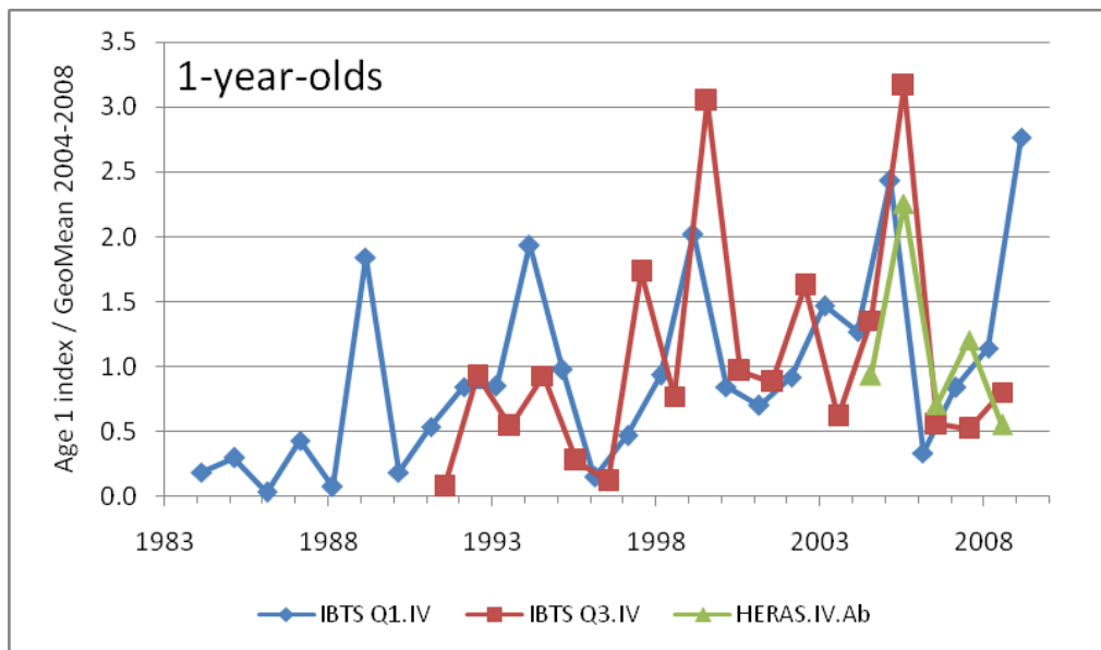
Figure 8.3.4. North Sea sprat. Normalized IBTS Q1, Quarter 3 and HERAS acoustic survey indices for age 1 North Sea sprat. All indices are normalized by their geometric mean over the common period from 2004-2008.
