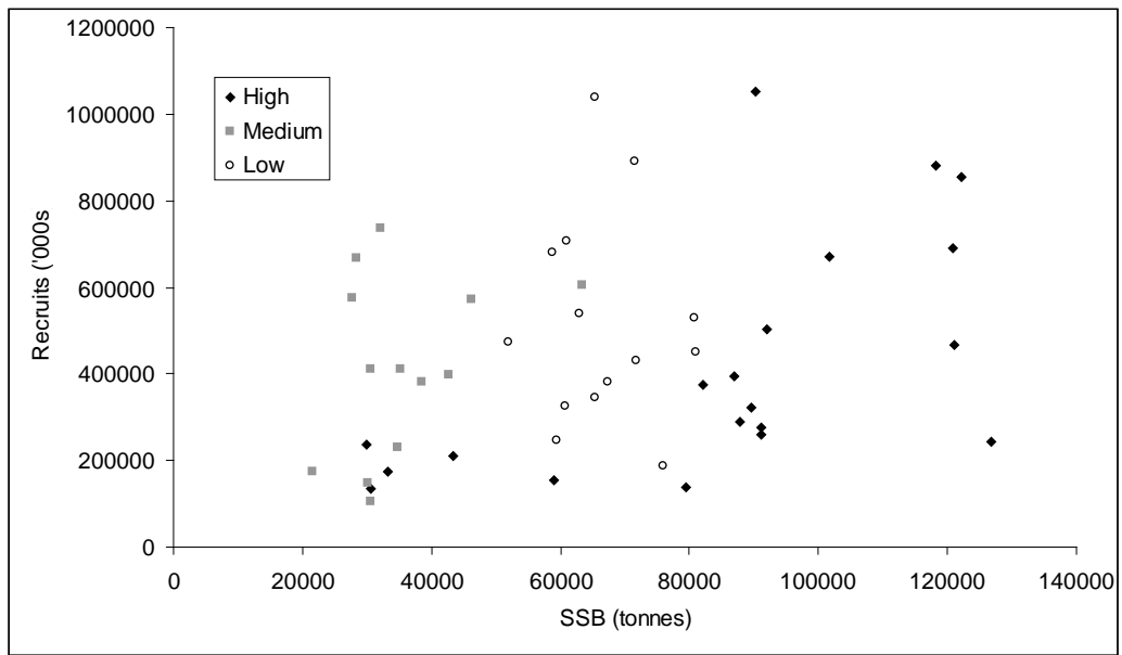
Figure 16. Herring in the Celtic Sea and VIIj. Stock recruit relationship from ICA base case runs. Data classified according to quality of input data, see Table 4.
