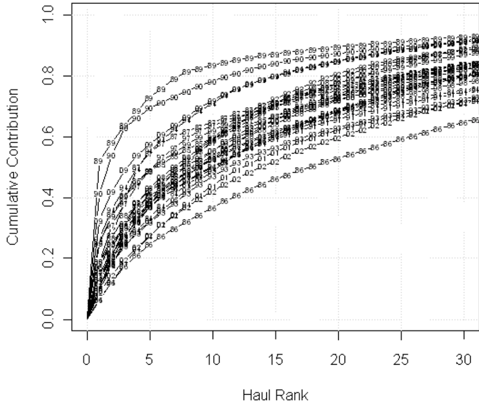
Figure 8.3.5 North Sea sprat. Normalized cumulative-distribution of the per-haul contribution to the IBTS q1 sprat age 1 survey index. The 300-450 individual hauls contributions to the IBTS index in each year are sorted by size and then aggregated to calculate a cumulative-distribution. The plot shows only the contribution for the 30 largest hauls. Numbers on each line indicate the year for the survey.
